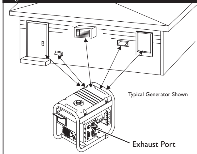
Figure 2 — Generator Clearance
